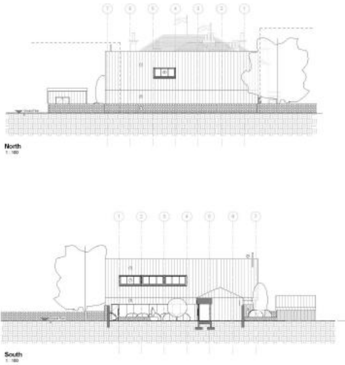
Fig 4 Proposed Elevation to Rear and Courtyard
