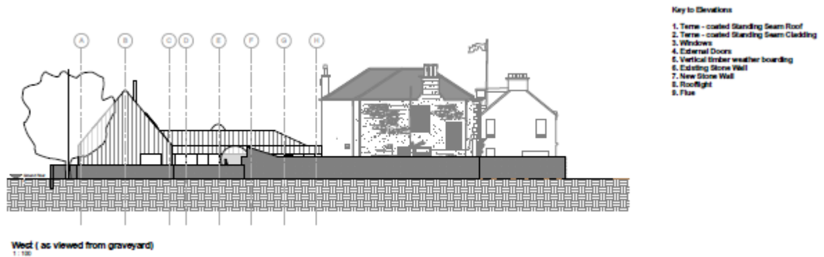
Fig 3 Proposed Elevation to Graveyard
