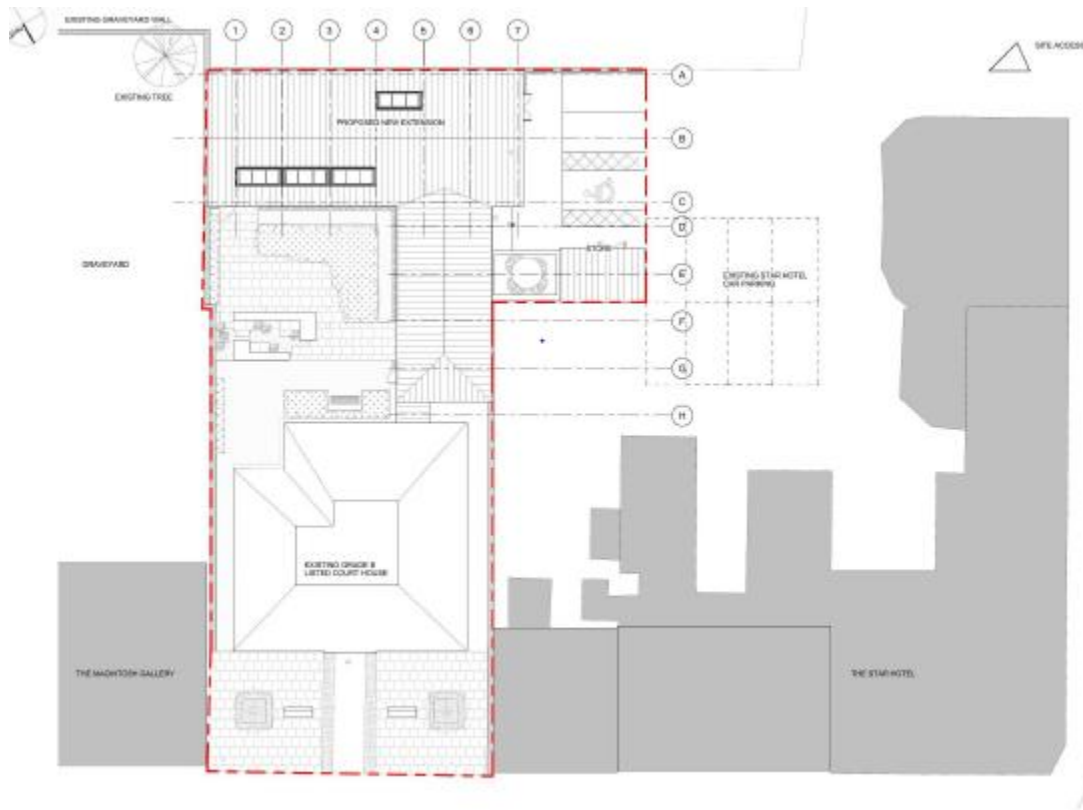
Fig 2 Proposed Site Layout
